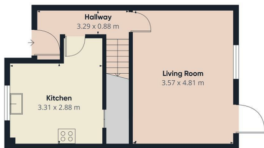
Floor 0
